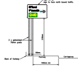
Detail 3.
